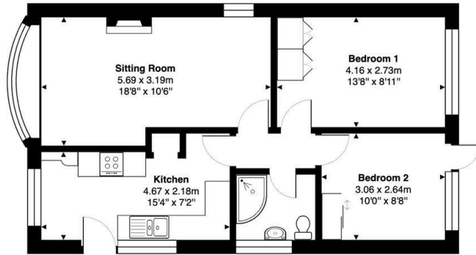
House Gross Internal Area: 55.6 m 2 ... 598 ft 2
